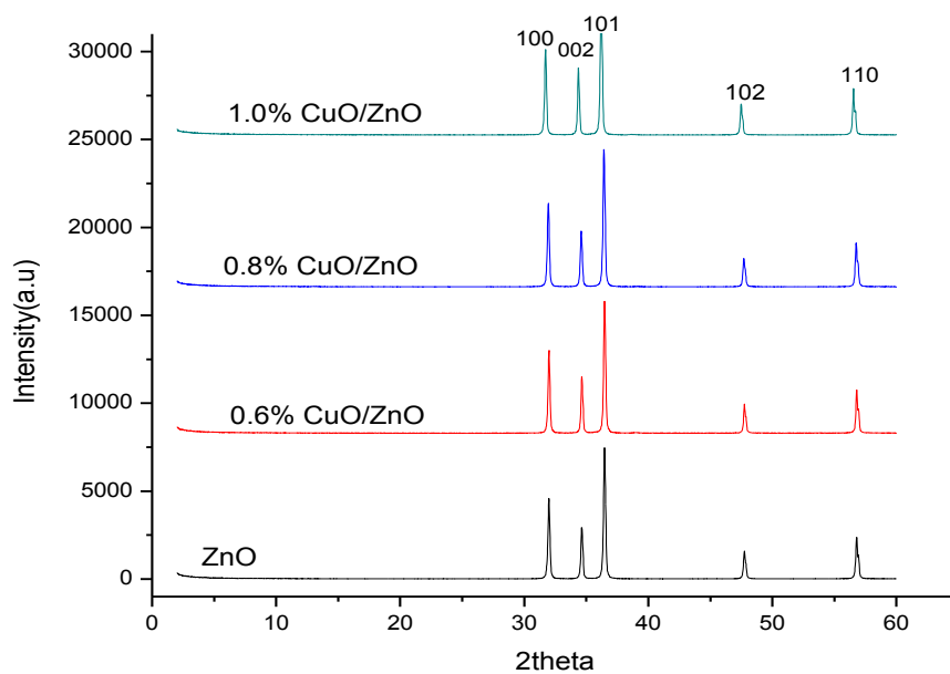
Figure 3. XRD diffractometer for ZnO and CuO/ZnO prepared with different percentage of CuO
