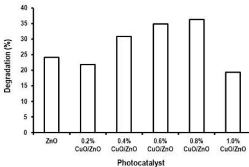
Figure 2. Photodegradation of methyl orange by ZnO and CuO/ZnO photocatalysts. Condition: mass of catalyst = 0.20 g, MO concentration = 10 ppm, pH = 6.8)
