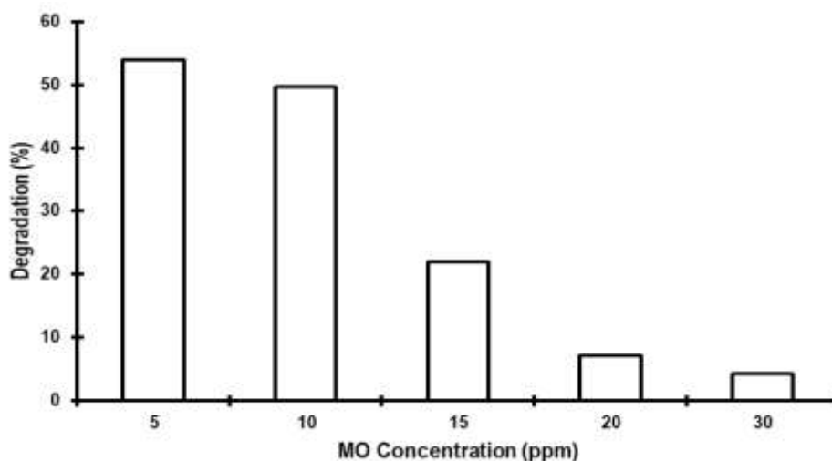
Figure 8. Photodegradation of MO of various concentrations by CuO/ZnO photocatalyst (Conditions: 0.6 g of photocatalyst, pH 6.8)
