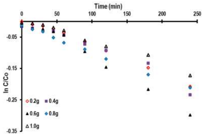
Figure 6. Kinetics of MO photodegradation at various amount of 0.8% CuO/ZnO catalyst (Conditions: 10 ppm MO; pH 6.8)
