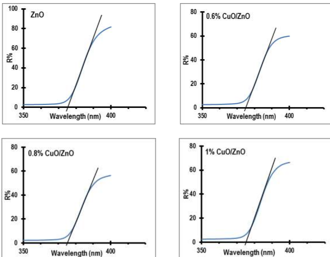
Figure 5. Diffuse reflectance UV-Vis spectra for ZnO and CuO/ZnO photocatalysts
