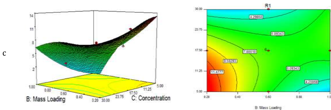
Figure 9. Three dimensional response surface plots showing the effect between a) Ph of MO solution and catalyst loading, b) pH and concentration of the MO solution and c) catalyst loading and concentration of MO solution on the amount of MO degraded
