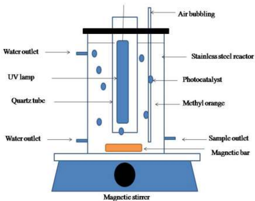
Figure 1. Schematic diagram of the photoreactor
