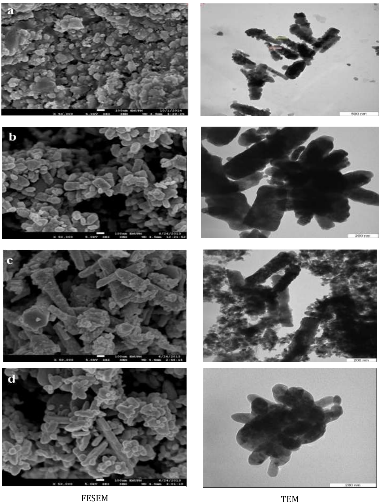
Figure 4. The FESEM and TEM images of a) ZnO, b) 0.6% ZnO/CuO, c) 0.8% ZnO/CuO and d) 1.0% ZnO/CuO
