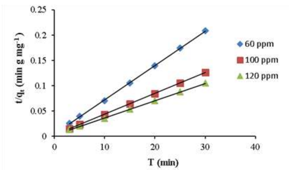
Figure 8. Plot of the pseudo second-order model at different initial nitrate concentration
