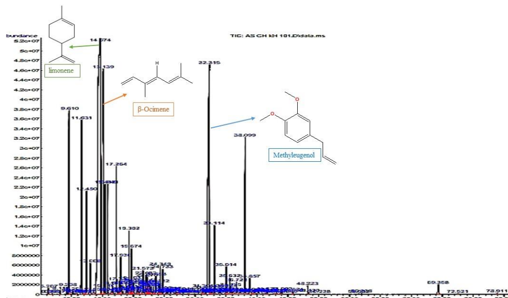
Figure 3. Chromatographic profile (GC/MS) of Chaerophyllum khorassanicum essential oils. The three major components are indicated, where (RT) from 14.5–15 (limonene), 15–15.5 (β-Ocimene), and 32–32.5 (methyl eugenol)
